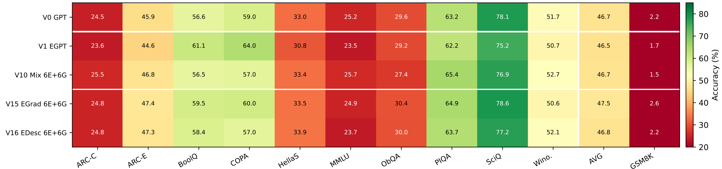
Output-rule ablation: V0/V1/V10/V15/V16 (all 12×1, d=768)
