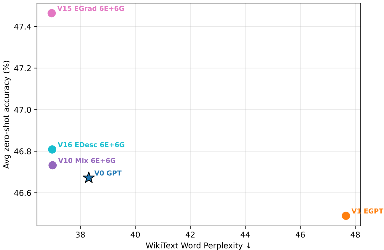
Accuracy vs Perplexity: output-rule ablation (all 12×1, 6E+6G heads unless labelled)
