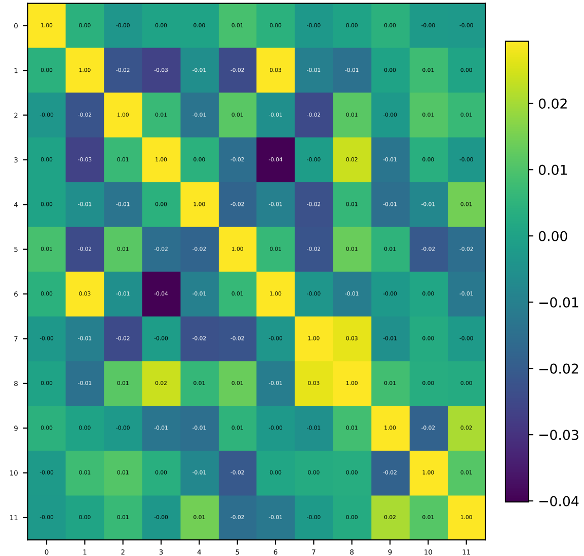
FFN sub-out \Delta
