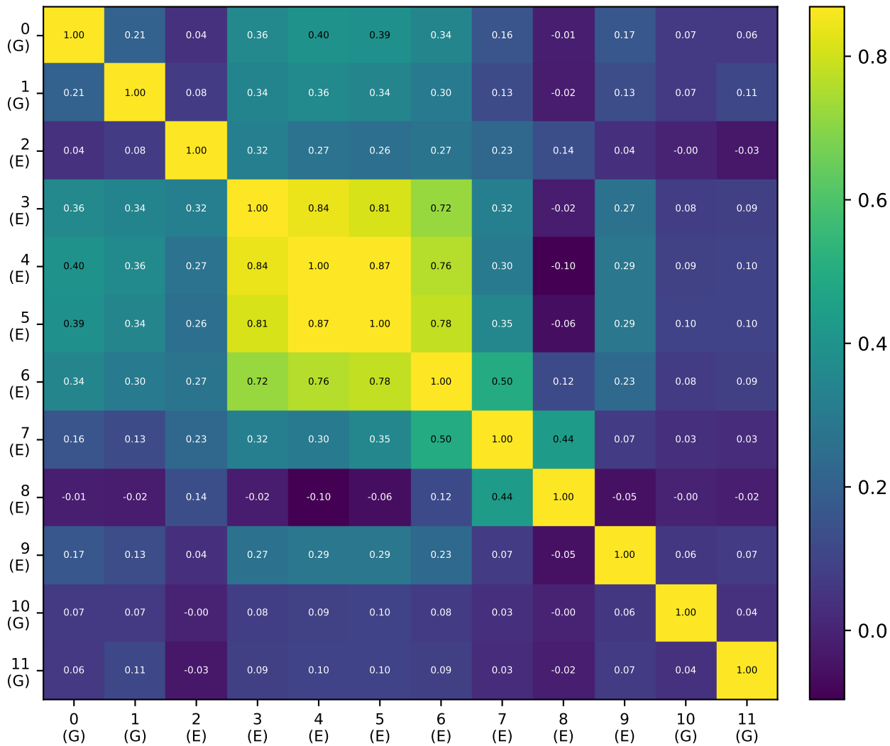
Same-input delta cosine sim — V41 Sandwich 2G+8E+2G
