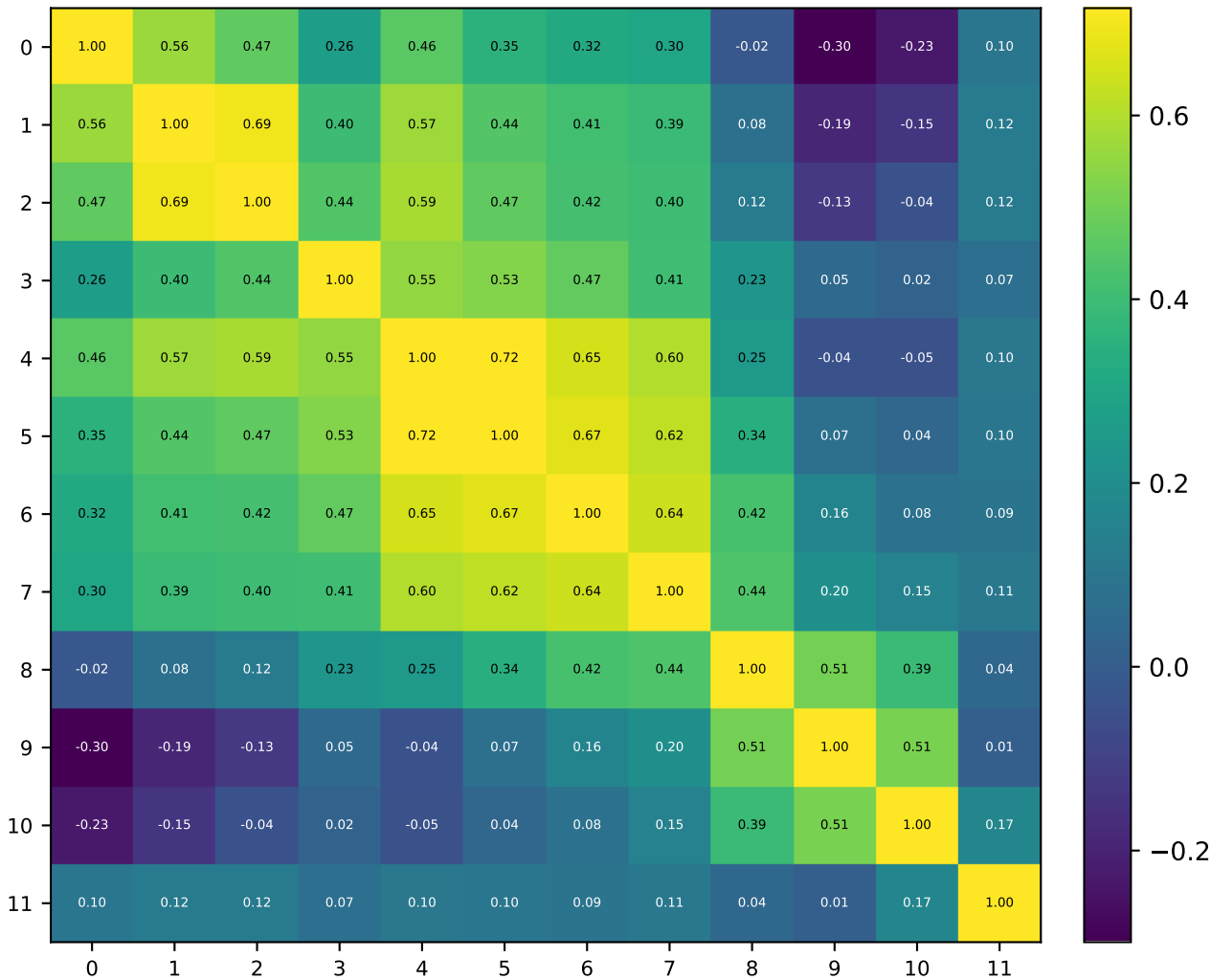
Same-Input Delta Cosine Sim — V1 EGPT 12×1 d768
