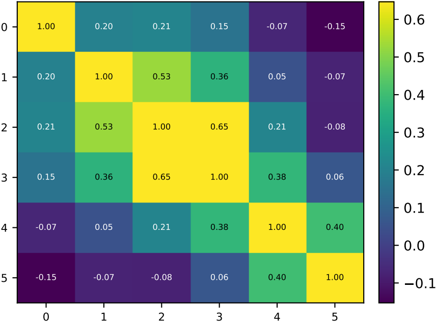
Same-Input Delta Cosine Sim — V43 Procrustes merge (init)
