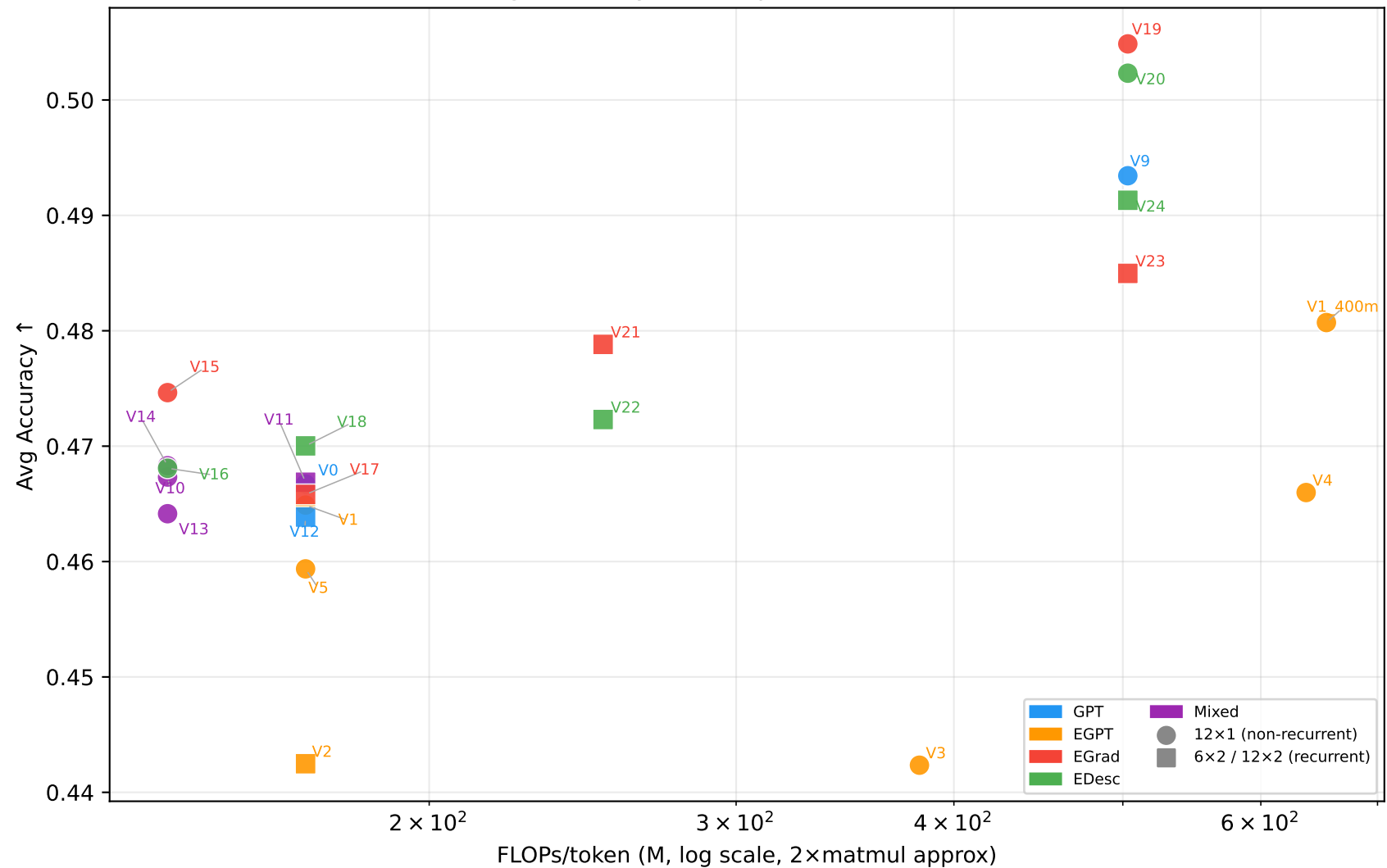
Avg Accuracy vs Compute (no Helmholtz)
