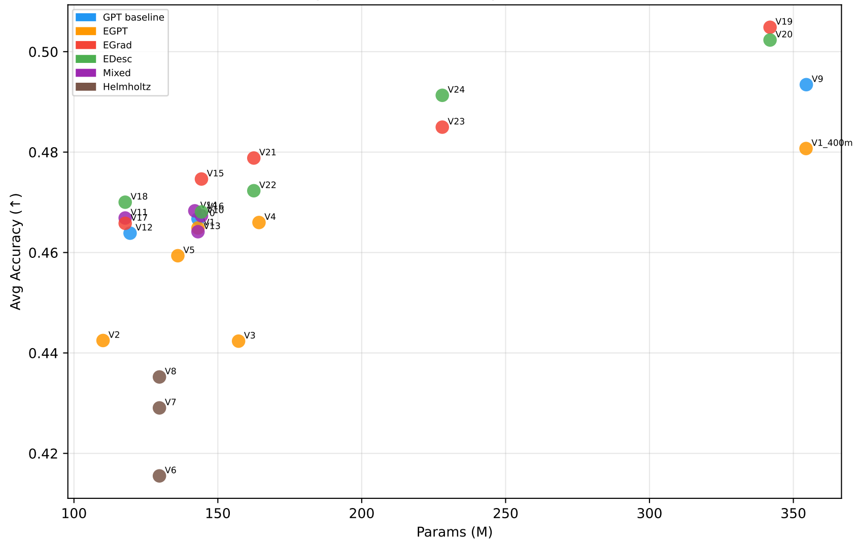
Avg Benchmark Accuracy vs Model Size
