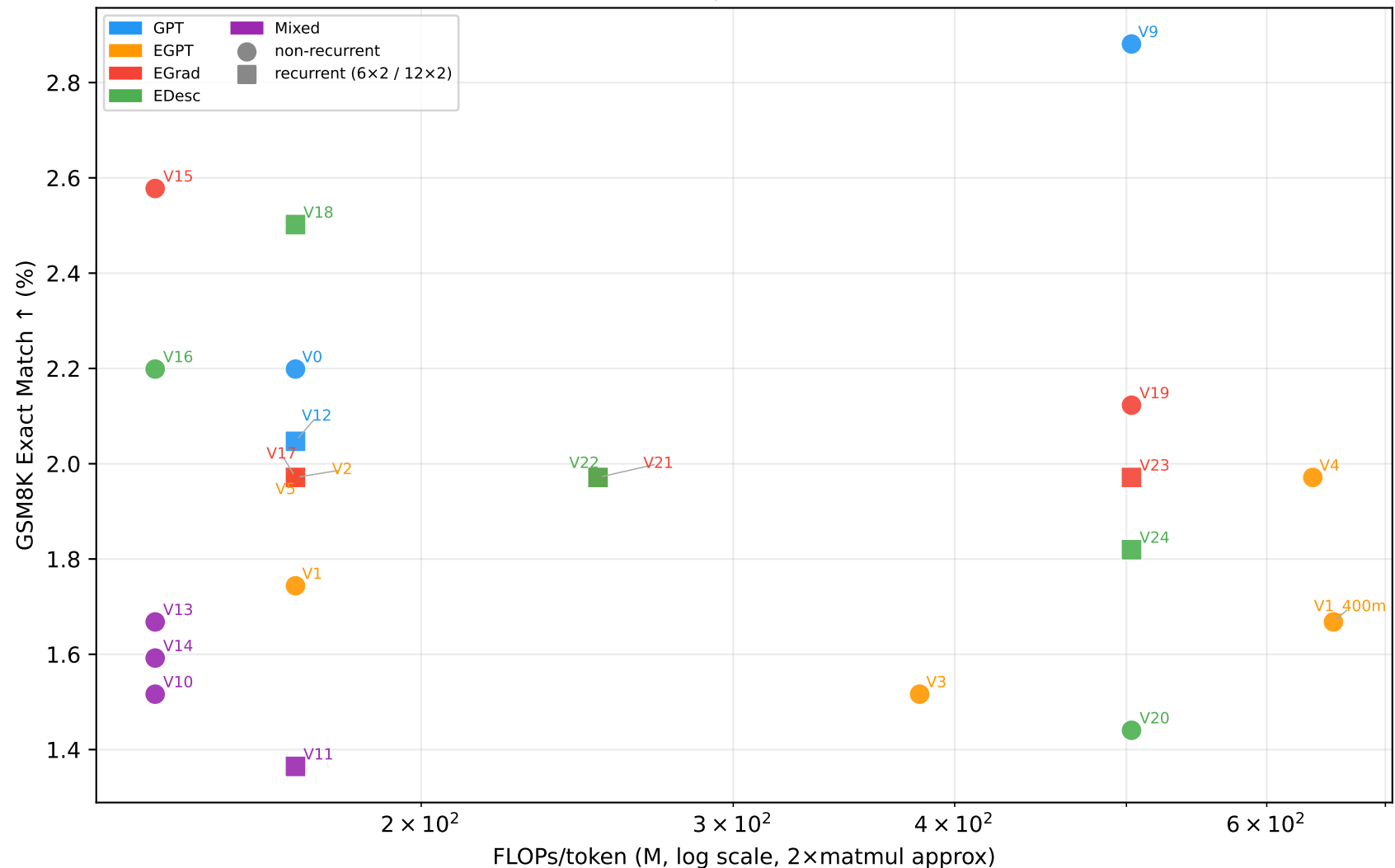
GSM8K vs Compute (no Helmholtz)
