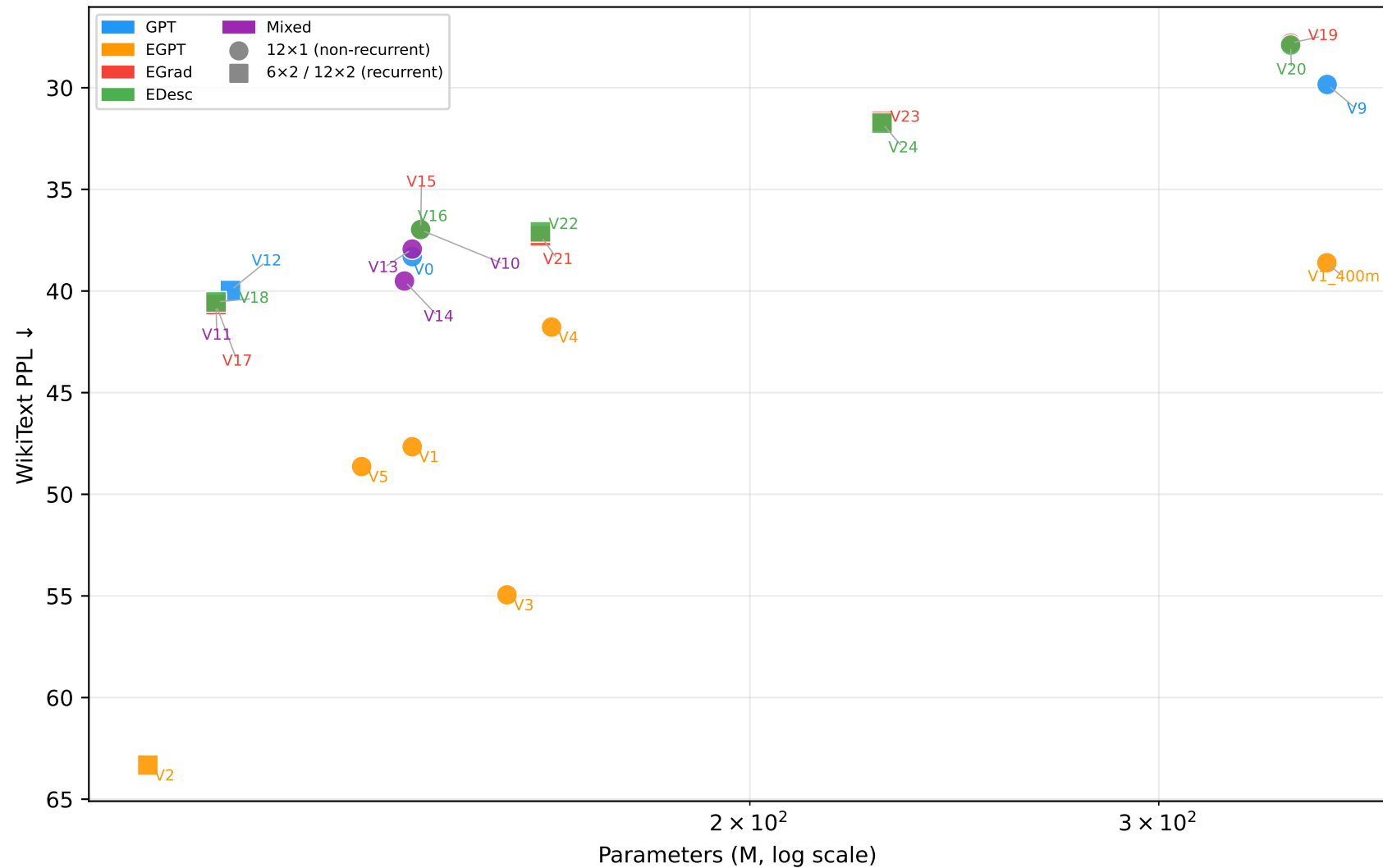
Perplexity vs Model Size (no Helmholtz)
