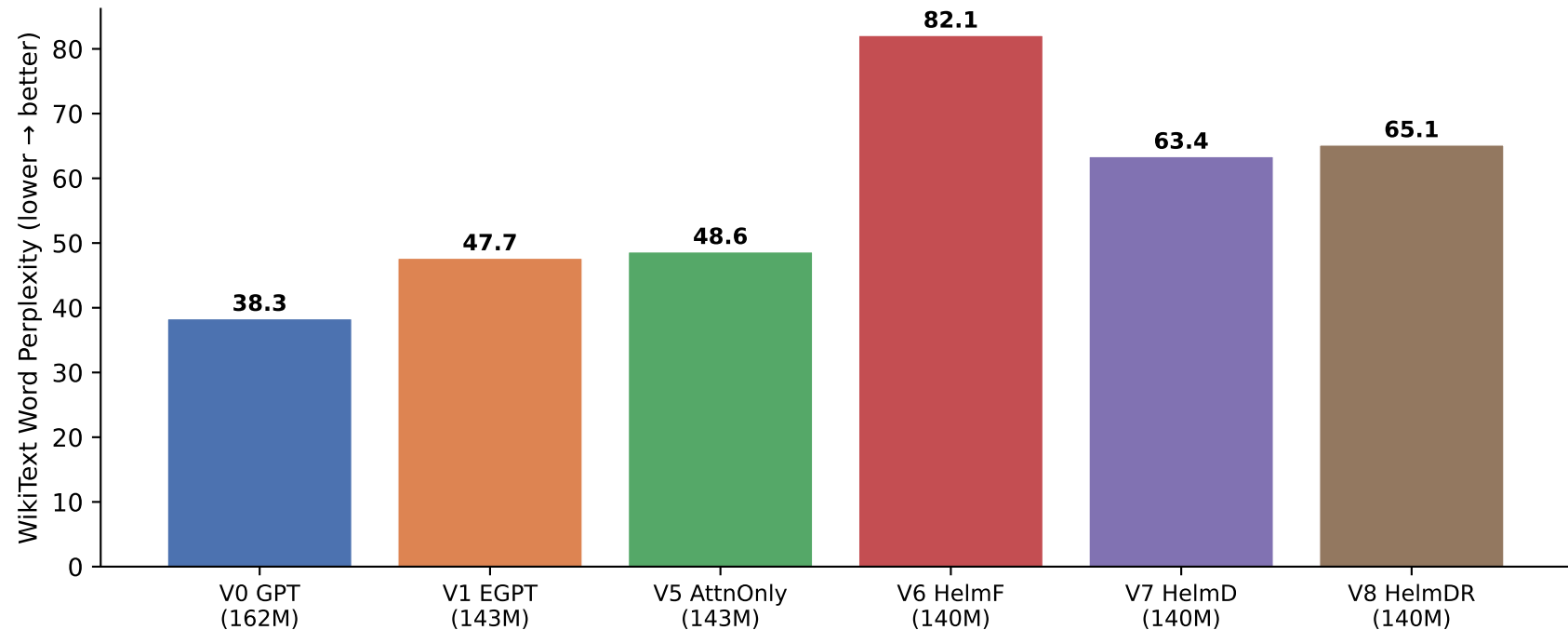
V5-V8 Ablation: WikiText Perplexity
