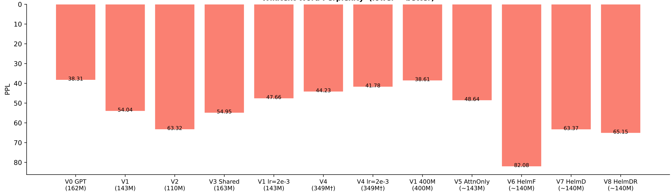
Wikitext Word Perplexity (lower → better)
