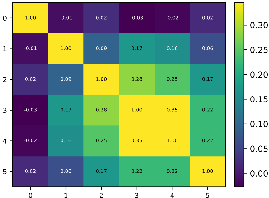
Attn Output Cosine Sim — V43 Procrustes merge (init)
