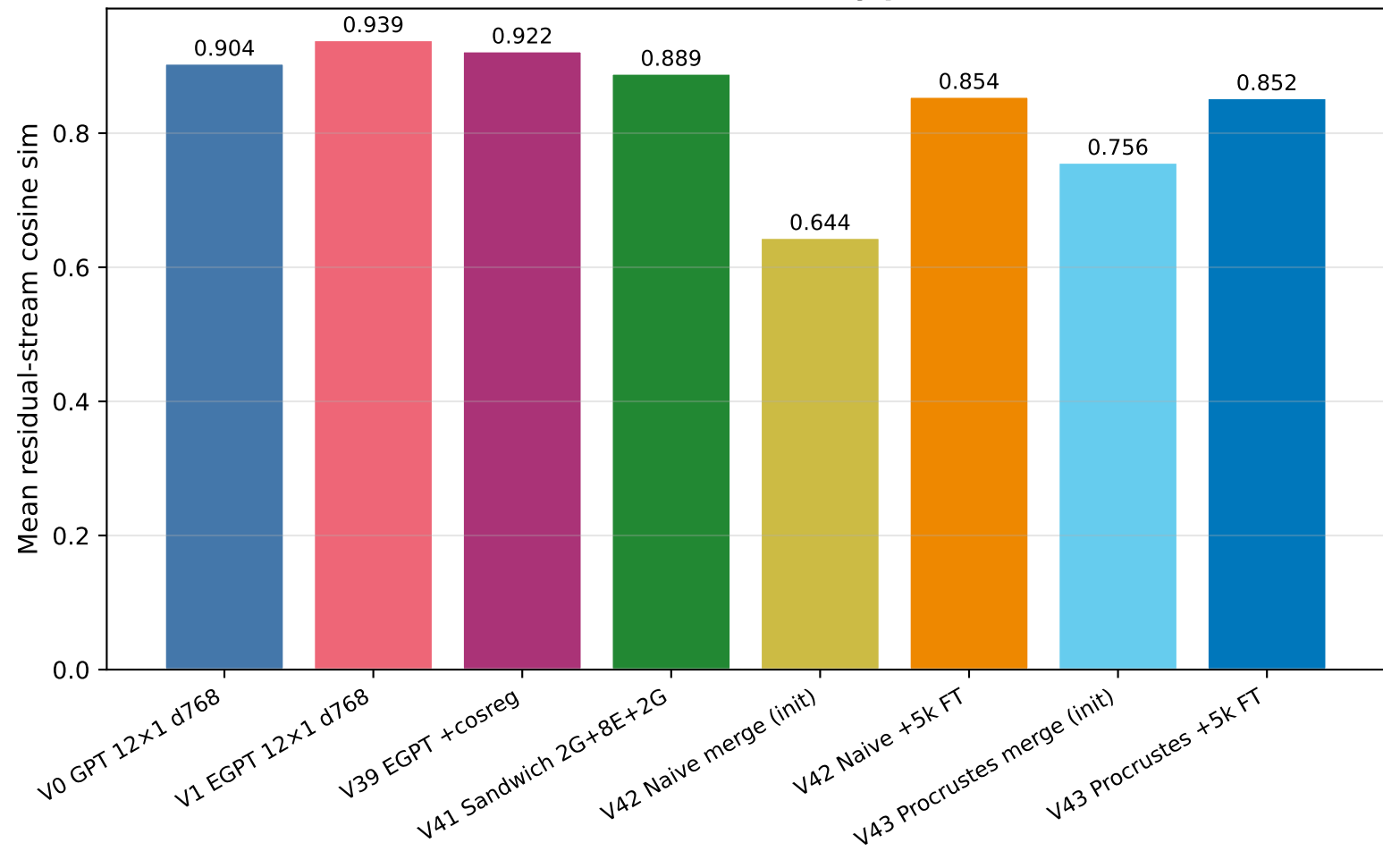
Mean Activation Similarity per Model
