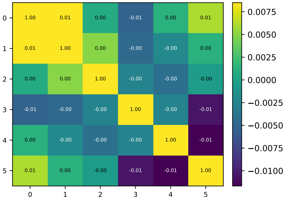
FFN Output Cosine Sim — V42 Naive +5k FT
