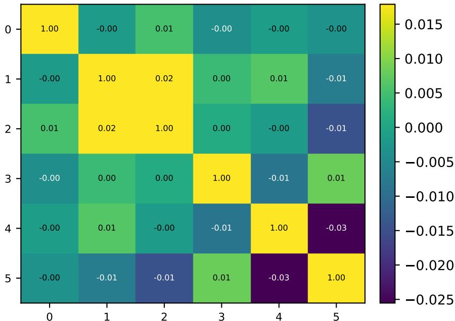
FFN Output Cosine Sim — V43 Procrustes merge (init)
