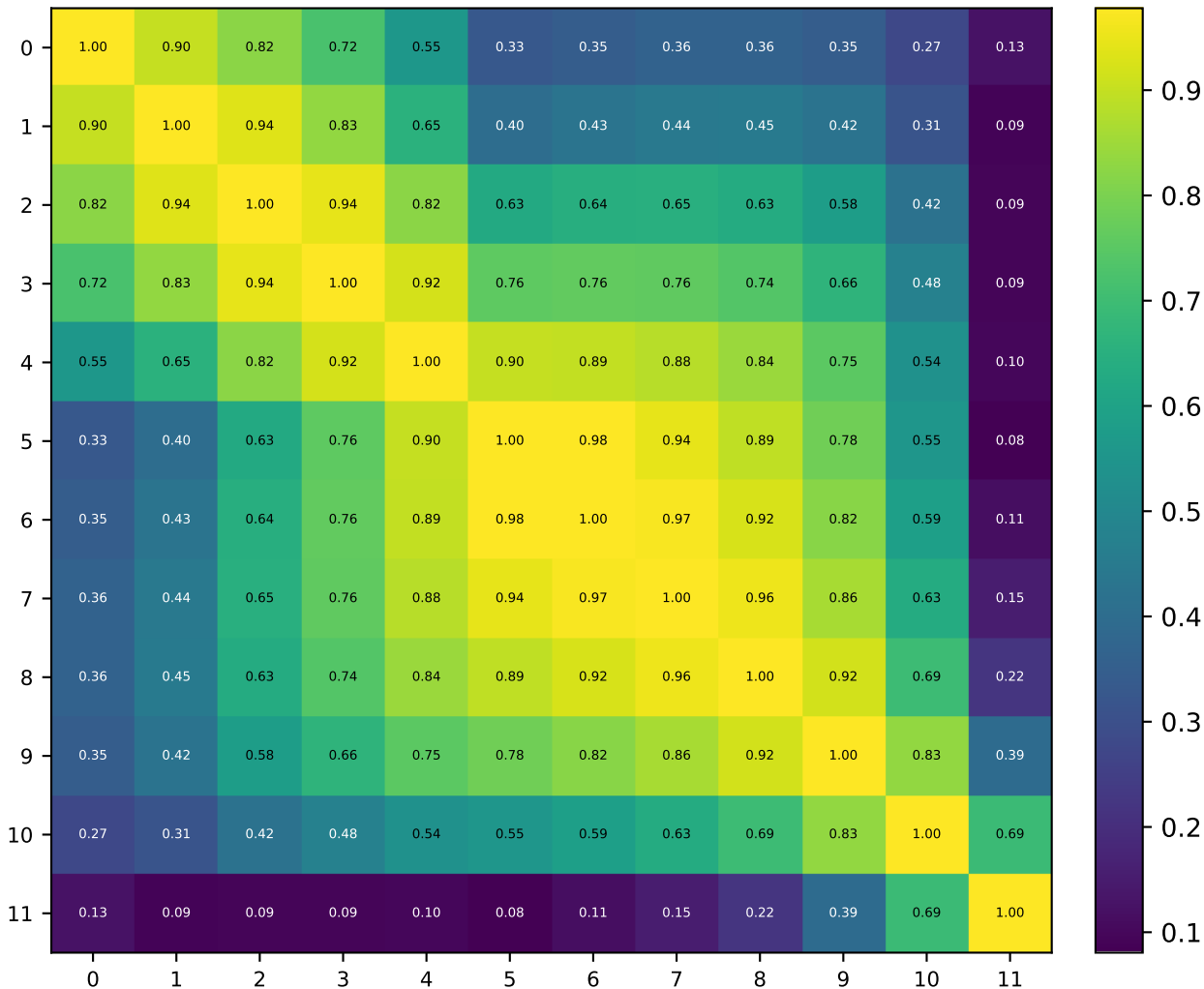
Residual-Stream Cosine Sim — V0 GPT 12×1 d768
