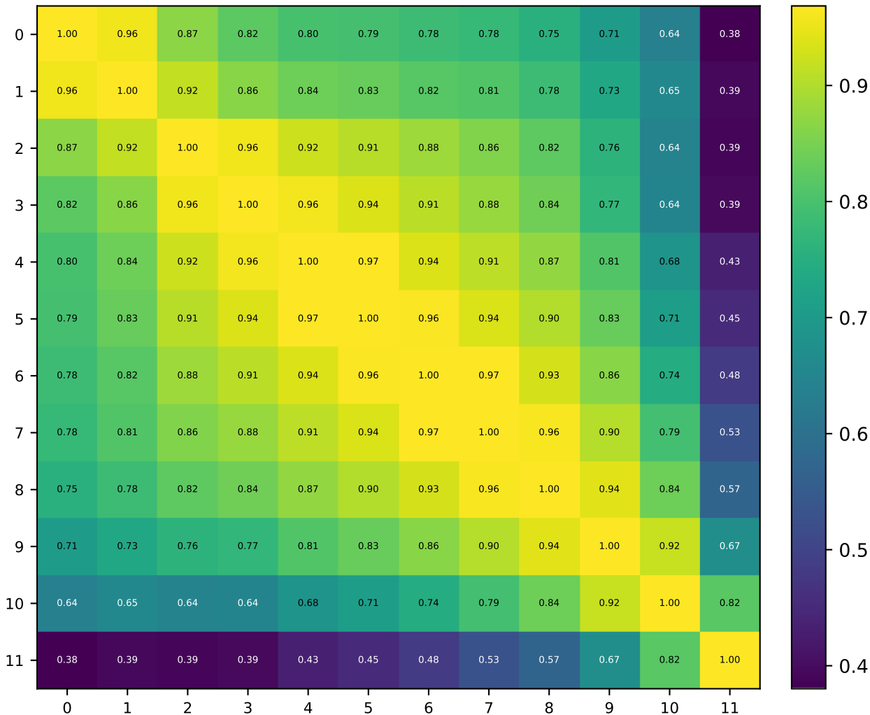
Residual-Stream Cosine Sim — V1 EGPT 12×1 d768
