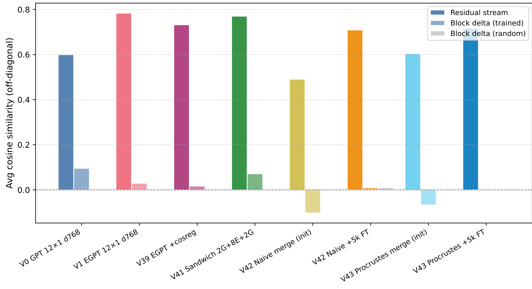
Residual-stream vs Block-delta vs Random Baseline
