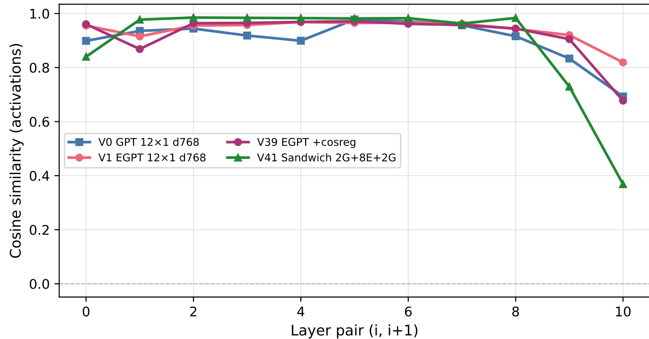
Residual-Stream Cosine Sim, Consecutive Layers (12-layer)
