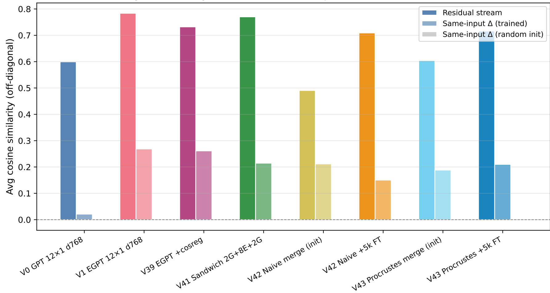
Layer similarity: residual vs same-input \Delta vs random baseline
