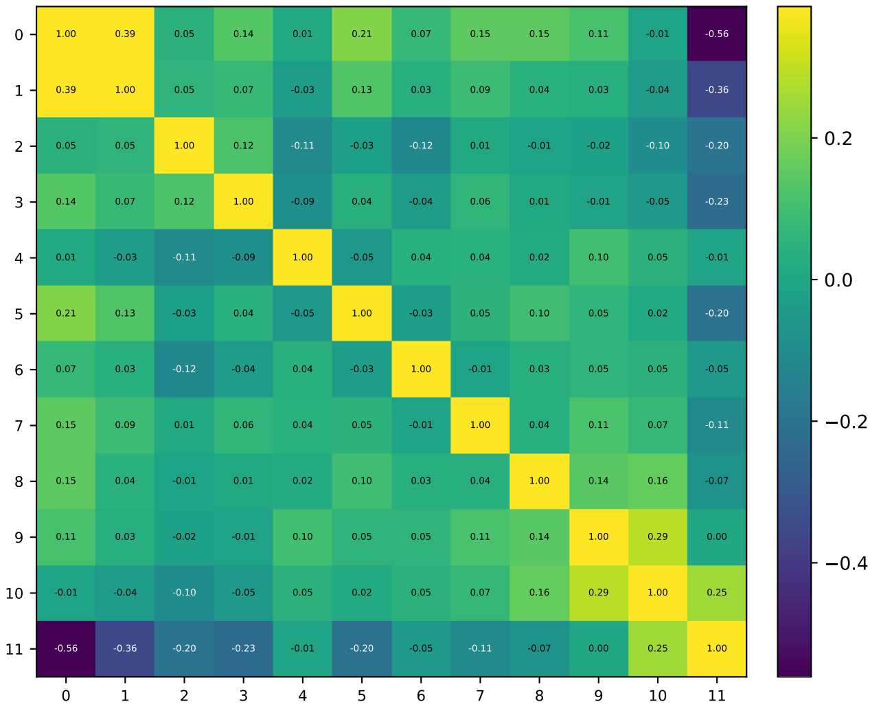
Block-Delta Cosine Sim — V39 EGPT +cosreg
