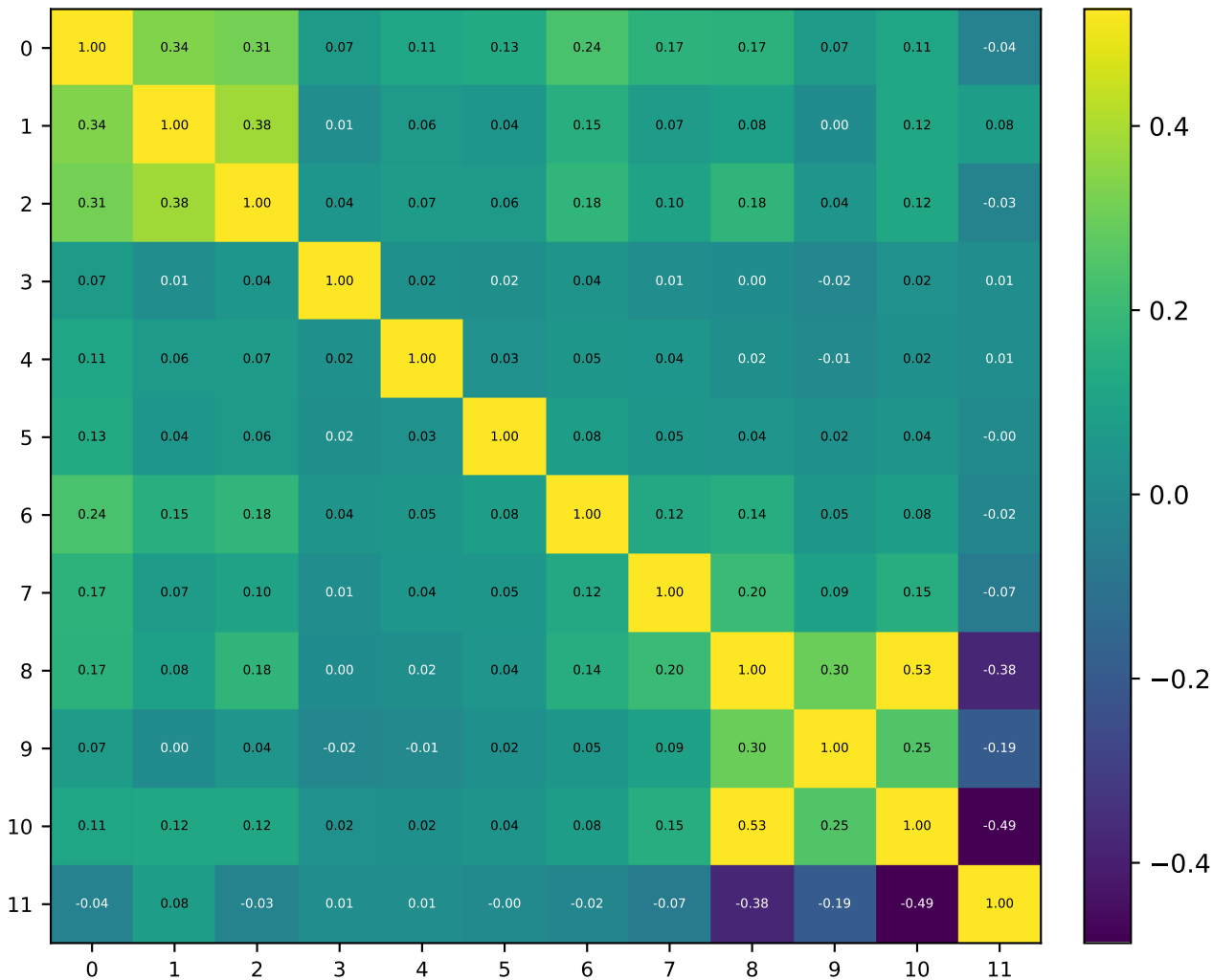
Block-Delta Cosine Sim — V41 Sandwich 2G+8E+2G
