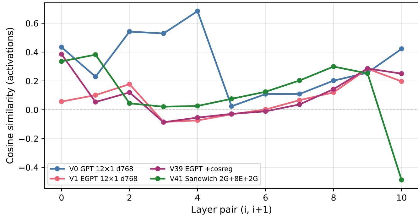
Block-Delta Cosine Sim, Consecutive Layers (12-layer)
