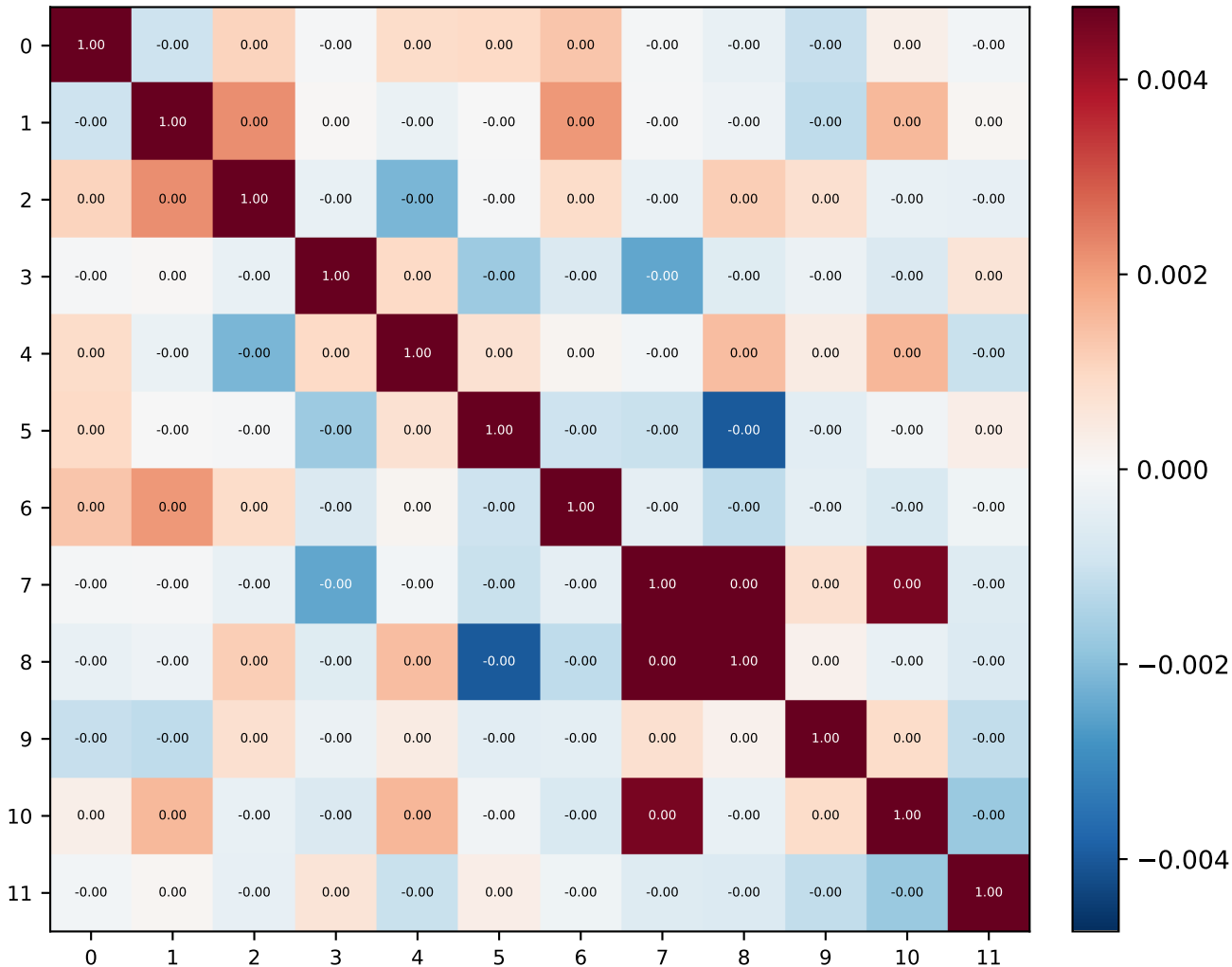
Attn Weight Cosine Sim – V0 GPT 12×1 d768
