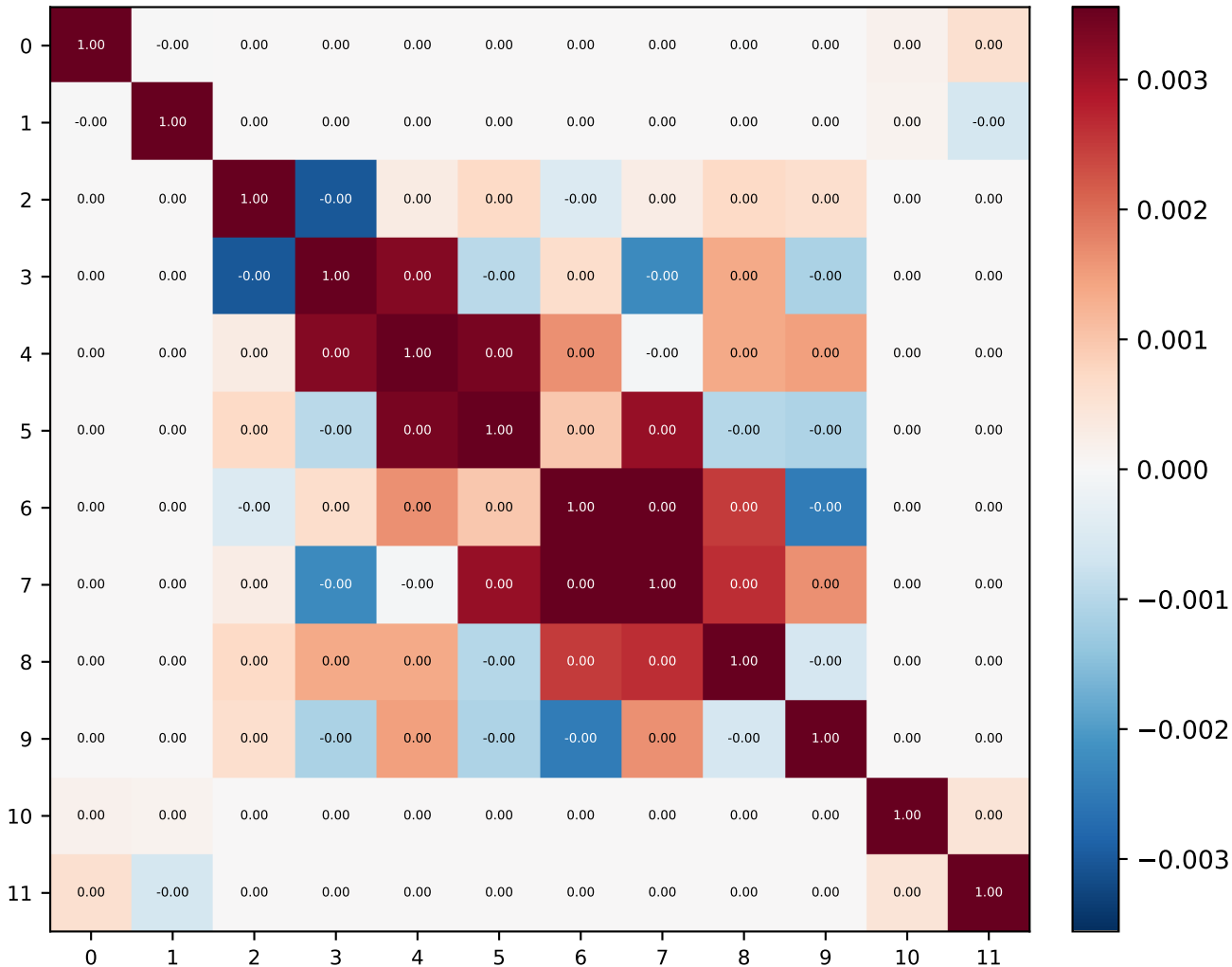
Attn Weight Cosine Sim — V41 Sandwich 2G+8E+2G
