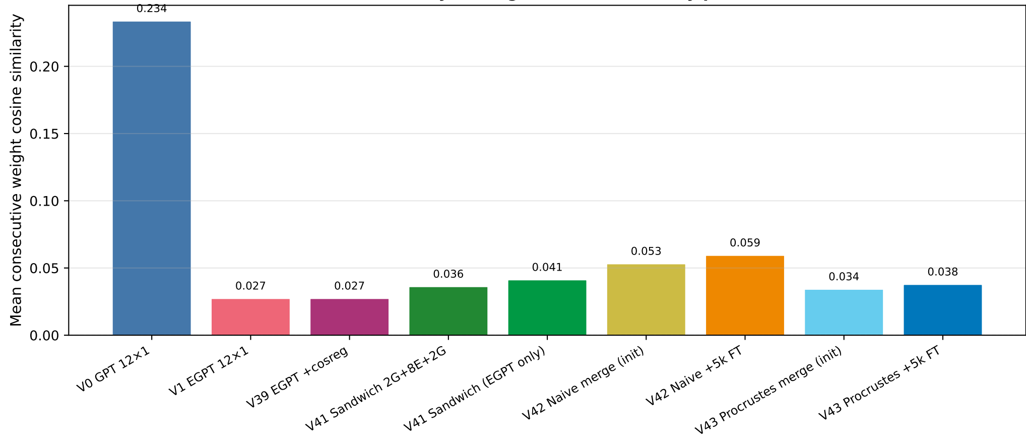
Consecutive-Layer Weight Cosine Similarity per Model
