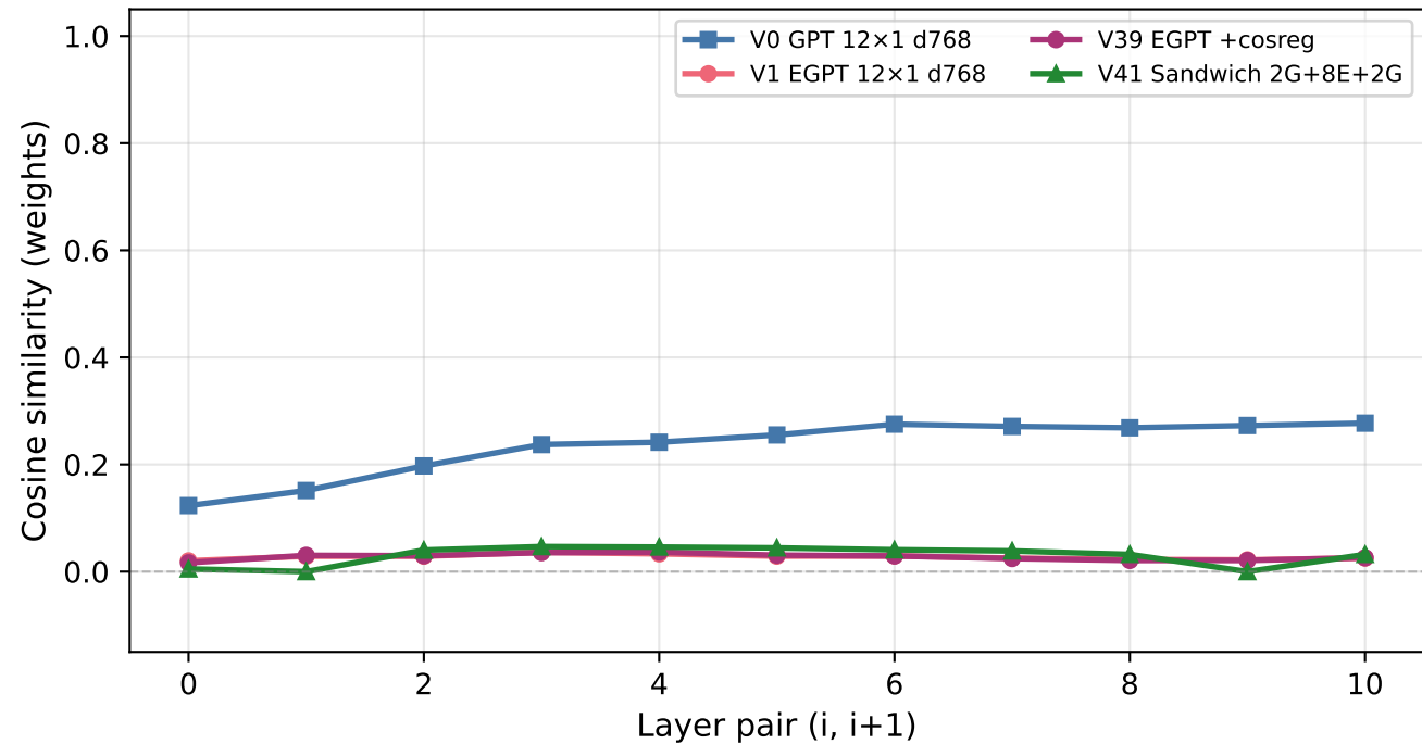
Weight Cosine Sim of Consecutive Layers (12-layer models)
