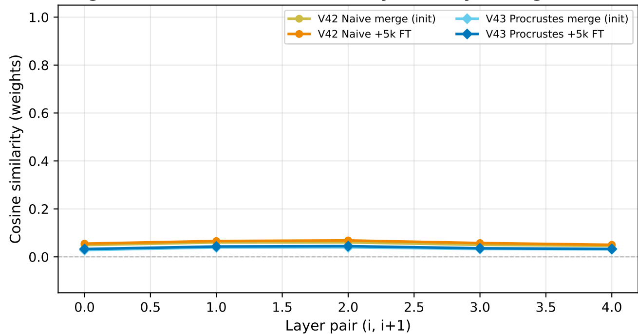
Weight Cosine Sim of Consecutive Layers (6-layer merged models)
