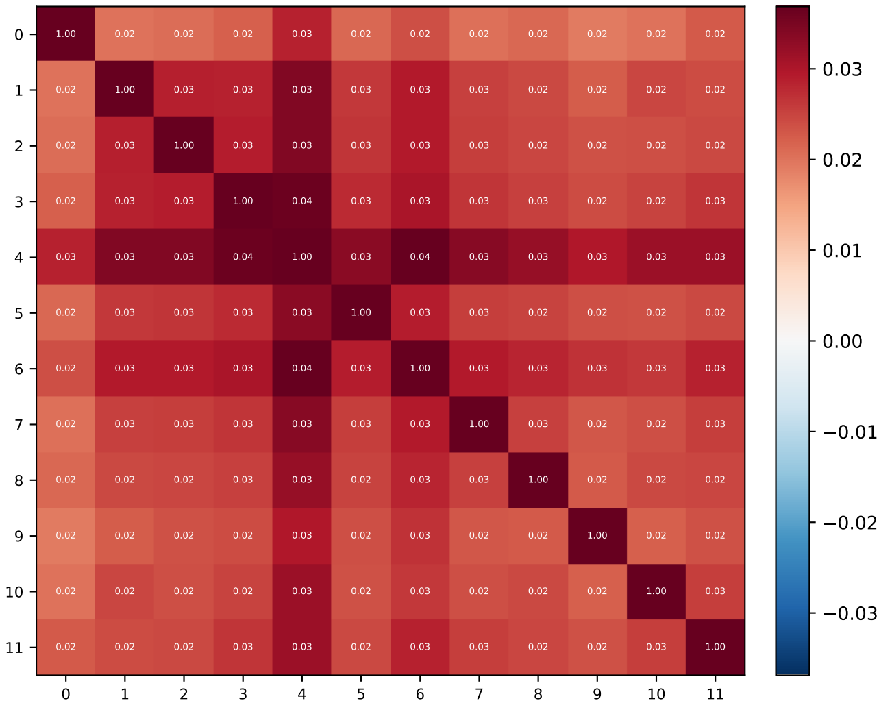
Weight Cosine Similarity — V1 EGPT 12×1 d768
