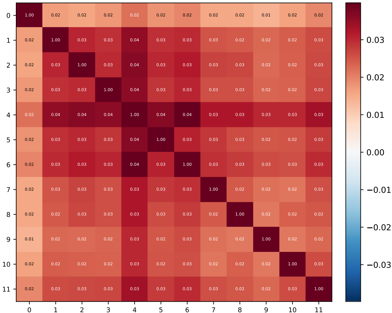
Weight Cosine Similarity — V39 EGPT +cosreg
