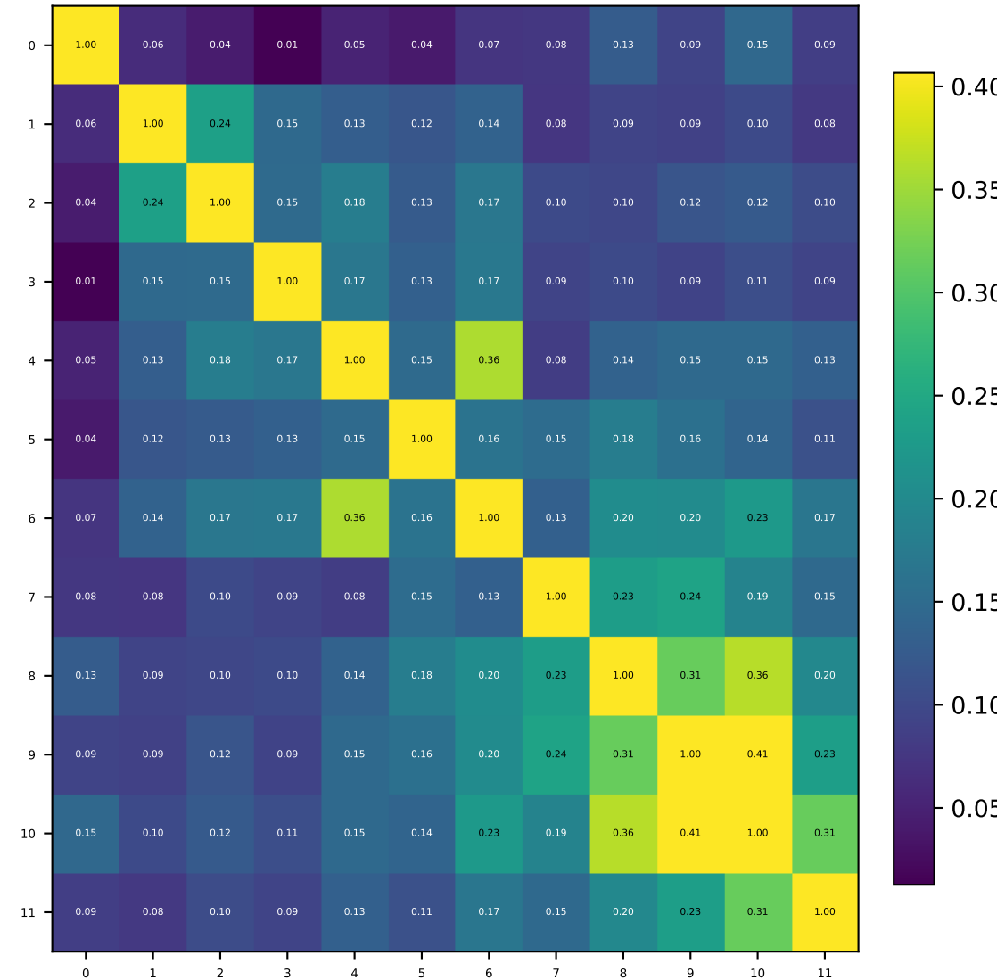
Attn sub-out \Delta
