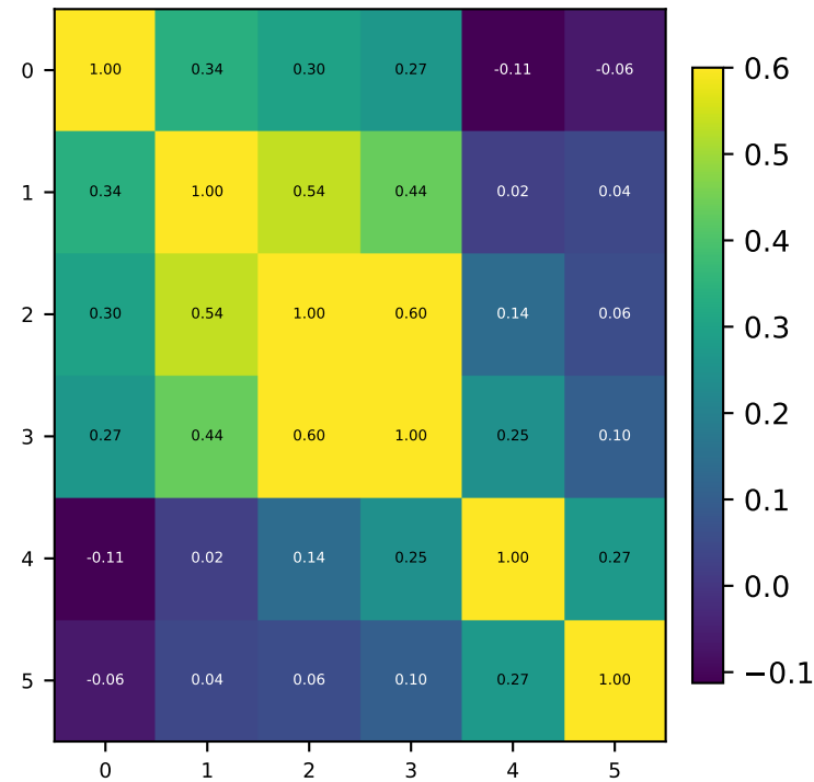
Full block \Delta
