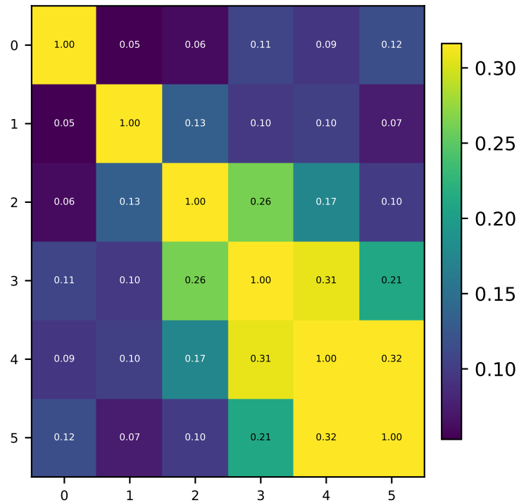
Attn sub-out \Delta
