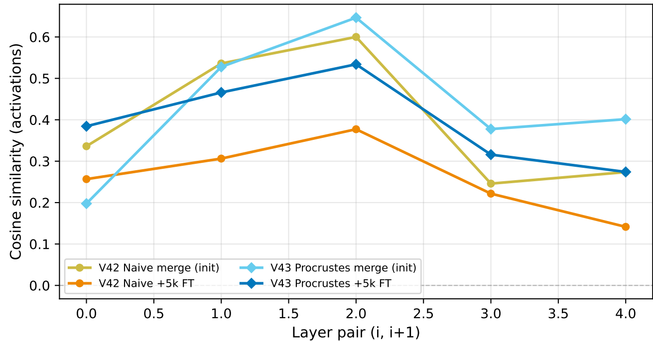
Same-Input Delta Cosine Sim, Consecutive Layers (6-layer merged)
