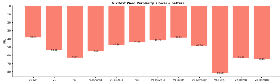
Figure 7: Summary metrics for early variants. V0 GPT (162M, 321 MFLOPs/tok) leads on perplexity; V1 EGPT lr=2e-3 (143M, 359 MFLOPs) nearly ties on accuracy despite the FLOPs gap.
