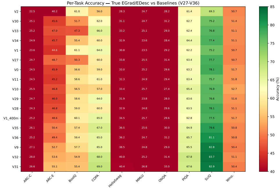
Figure 9: Per-task accuracy heatmap for true EGrad/EDesc vs. baselines. V27–V34 (red/green rows) show no systematic per-task advantage over Mixed or GPT.
