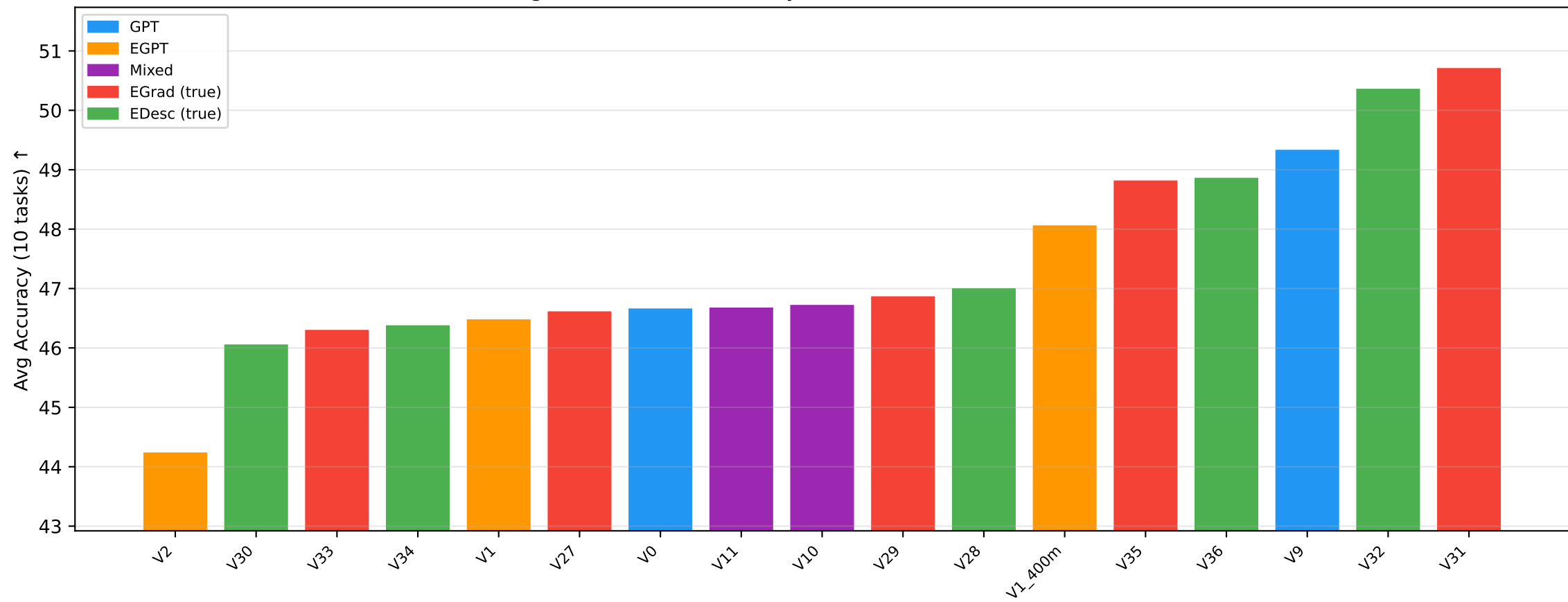
Average Benchmark Accuracy — True EGrad/EDesc vs Baselines
