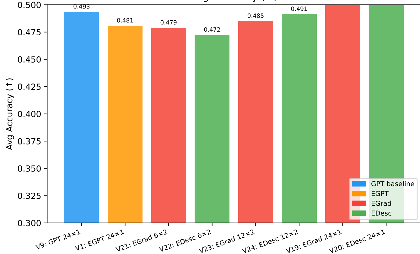
Avg Accuracy (↑)
