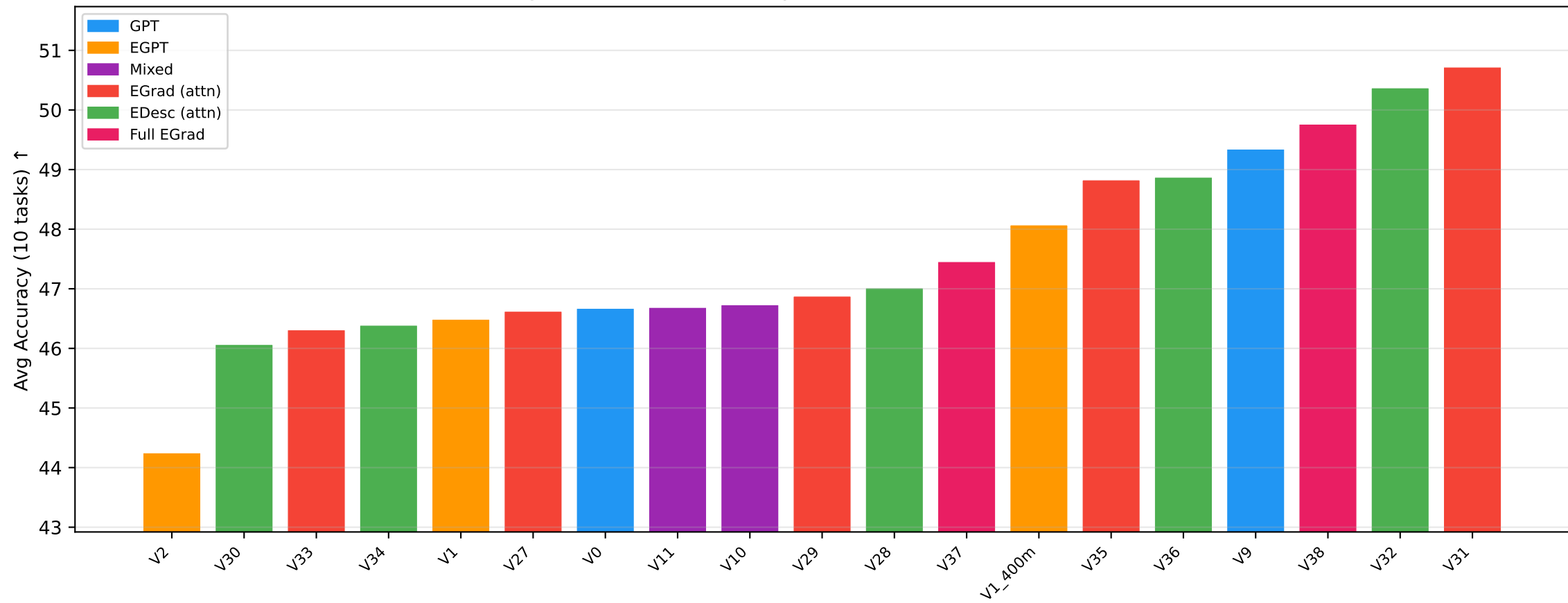
Average Benchmark Accuracy — EGrad(attn)/EDesc vs Baselines
