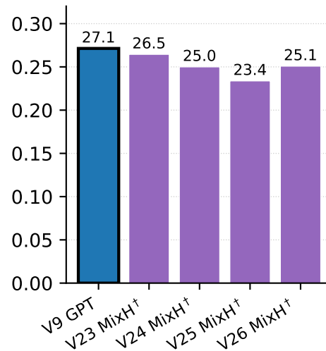
ARC-C
