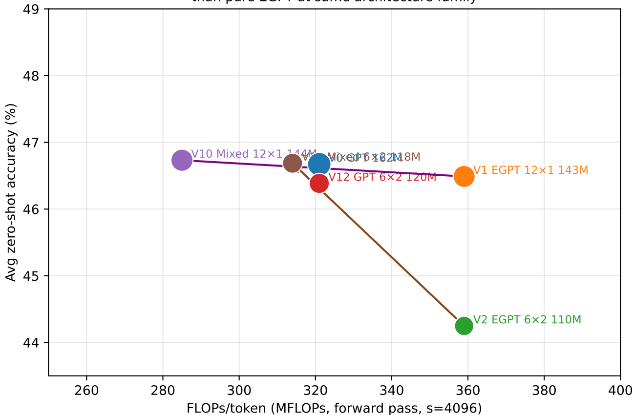
Accuracy vs Compute: Mixed heads are strictly more efficient than pure EGPT at same architecture family
