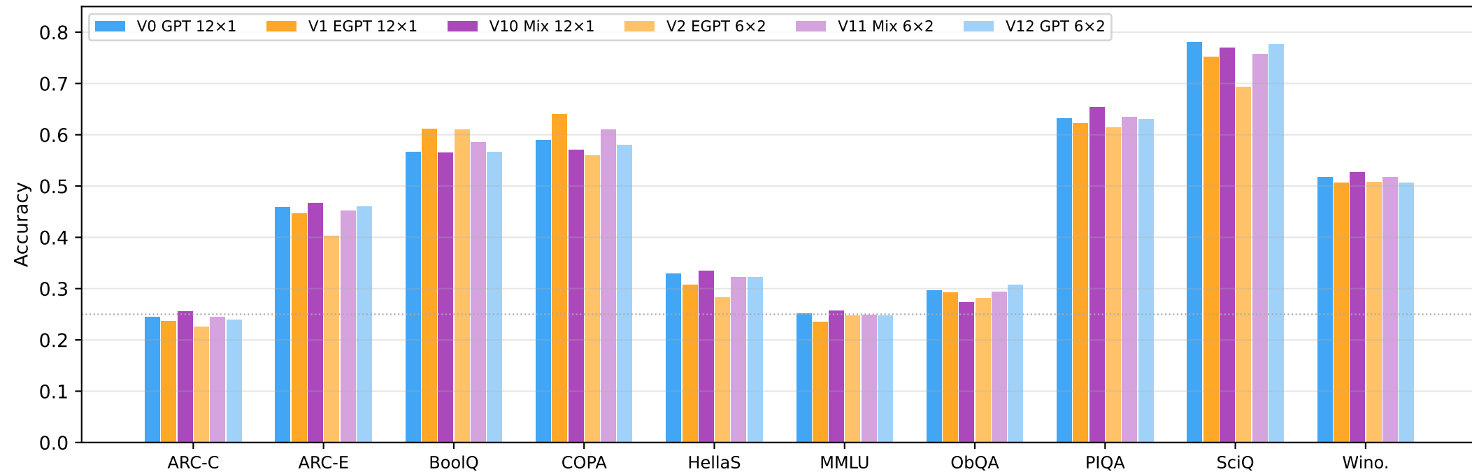
Iso-family comparison: non-recurrent 12×1 vs recurrent 6×2 — per task
