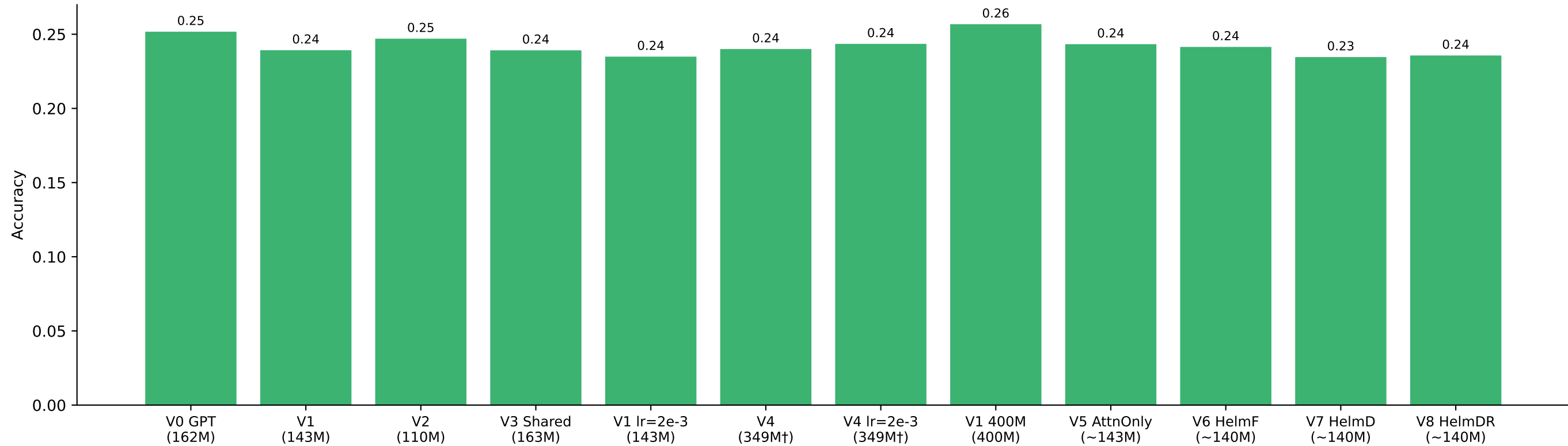
MMLU Accuracy
