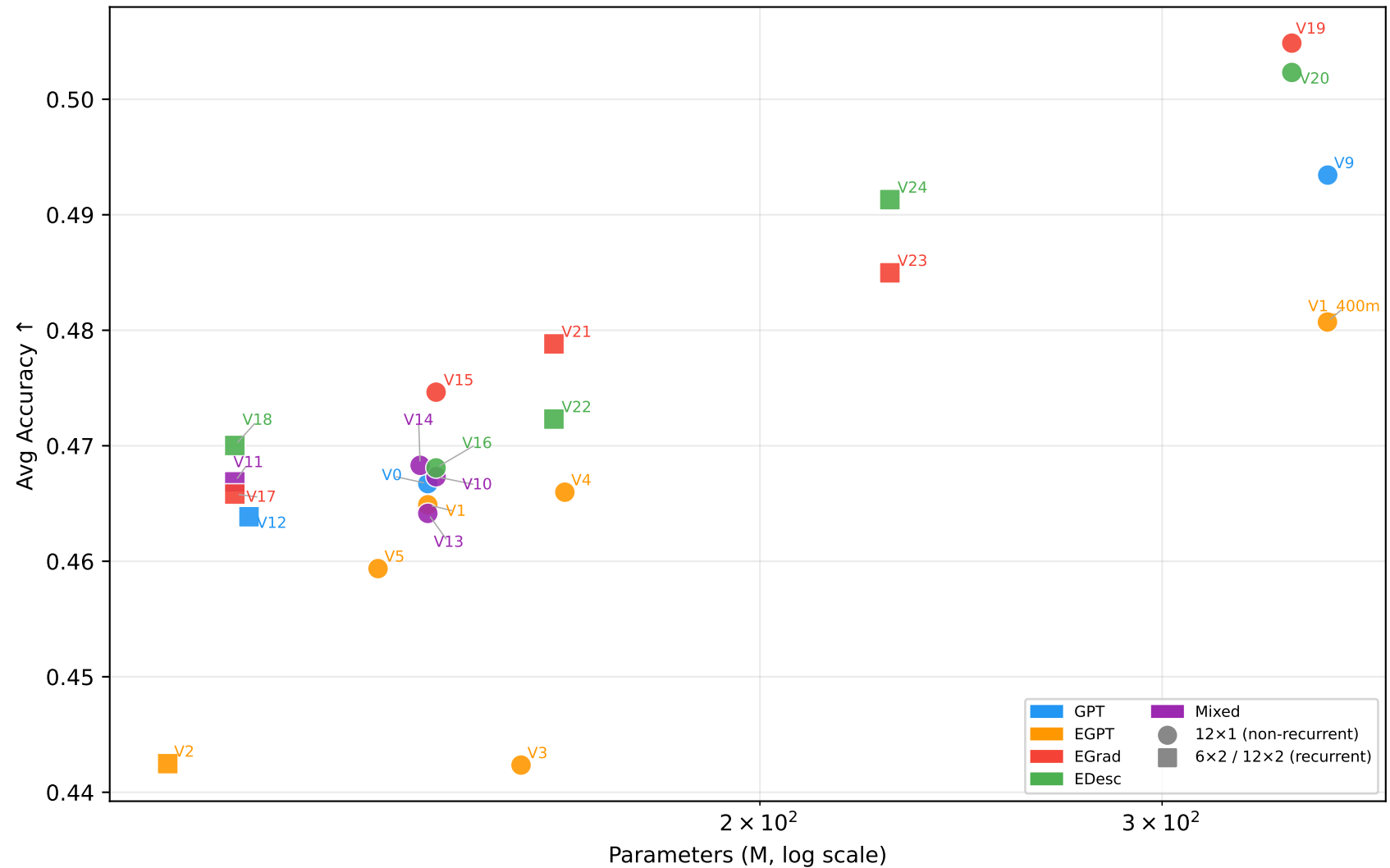
Avg Benchmark Accuracy vs Model Size (no Helmholtz)
