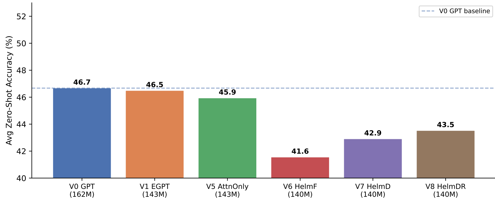
V5-V8 Ablation: Average Zero-Shot Accuracy (9 tasks)
