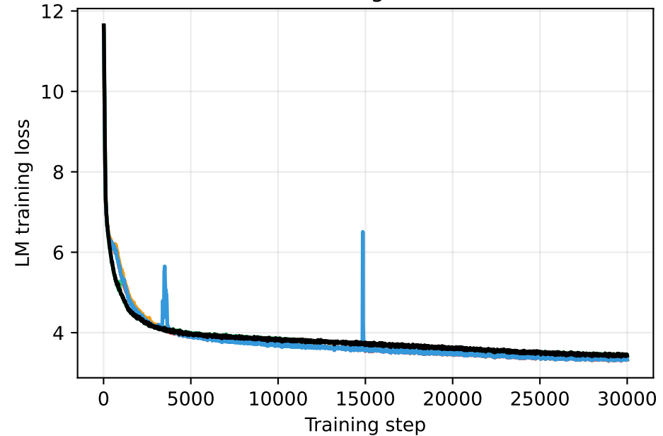
Training loss
