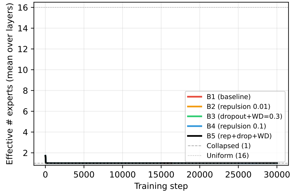
Routing diversity over training
