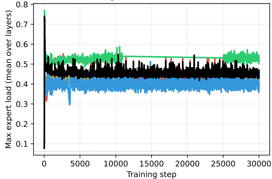
Expert load imbalance
