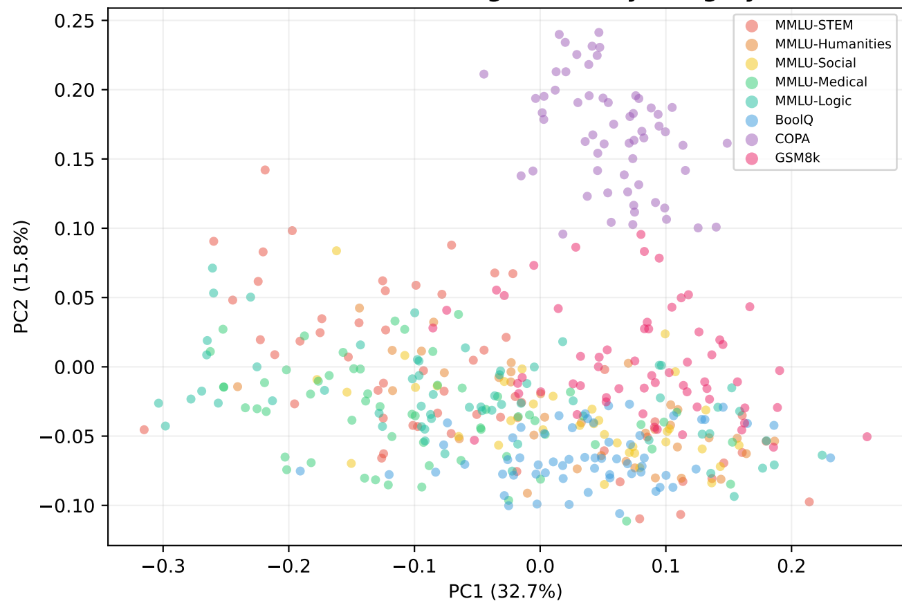
b5 — PCA of routing vectors by category
