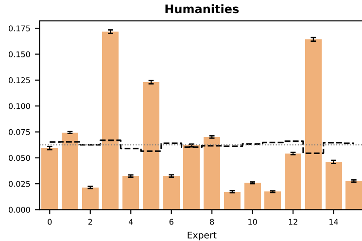
b1 — mean routing weight per expert by category (dashed = residual after subtracting global mean)
