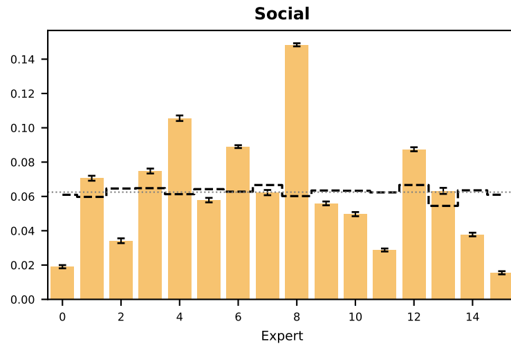
b2 — mean routing weight per expert by category (dashed = residual after subtracting global mean)
