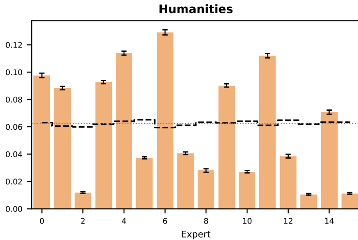
b3 — mean routing weight per expert by category (dashed = residual after subtracting global mean)
